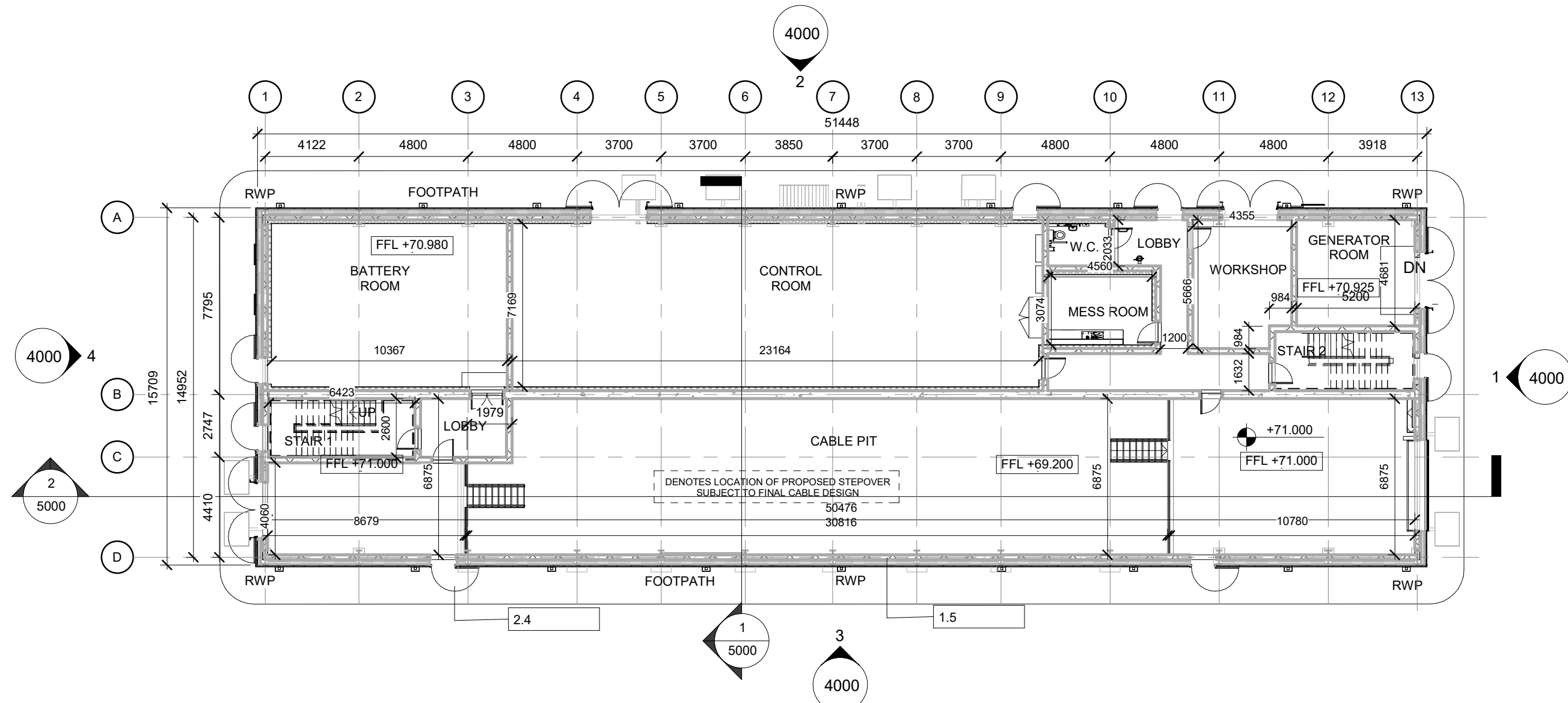
1 GROUND FLOOR PLAN 1 : 200
