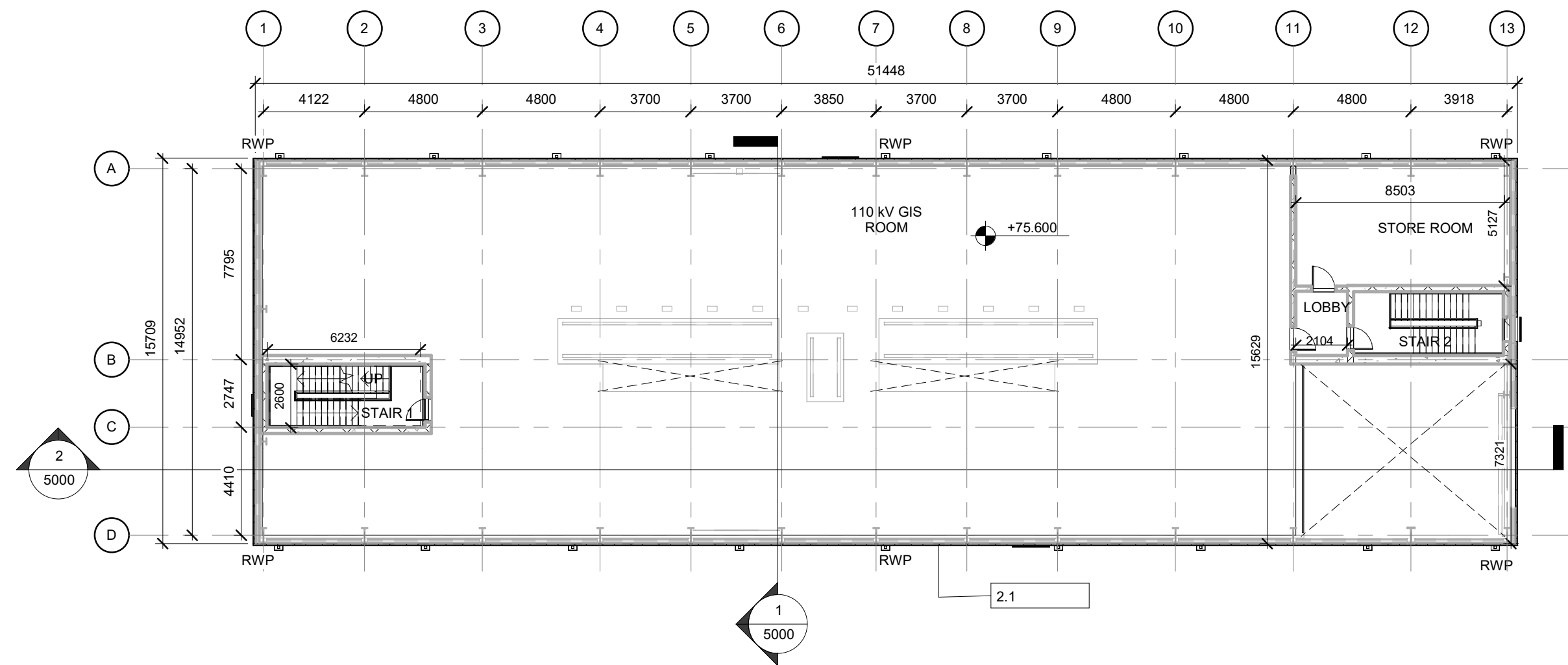
2 FIRST FLOOR PLAN 1 : 200
